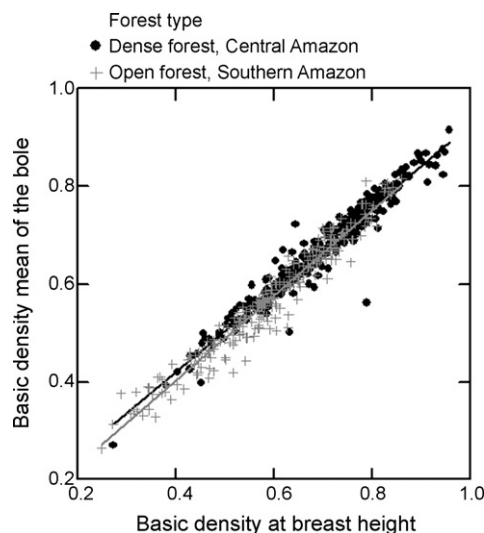
Fig. 4. Relationships between the mean basic wood density of the bole and wood density at breast height (full disk) in dense forest in central Amazonia ( n = 307 ) and in open forest in southern Amazonia ( n = 235 ).
