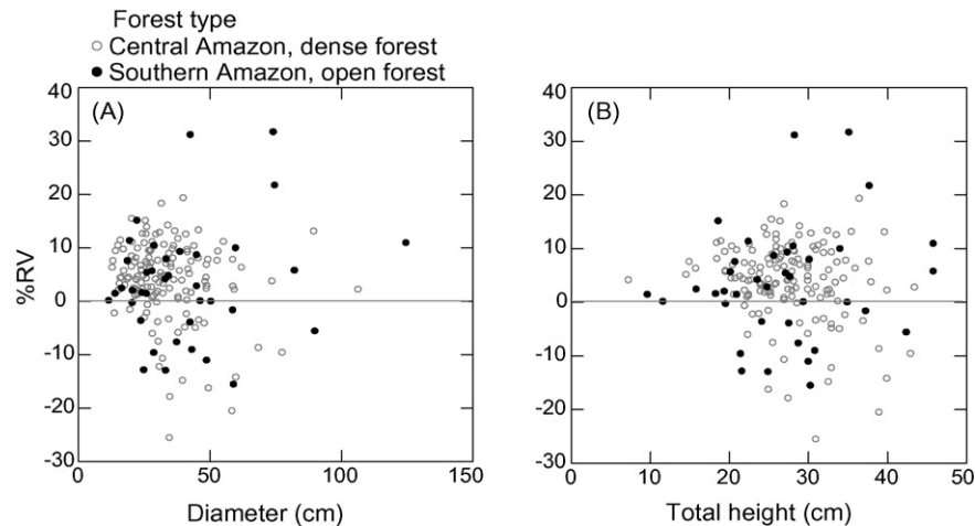
Fig. 3. Relationships between diameter (at breast height or above buttresses) and total height of trees with %RV (meaning the percentage difference between basic density of heartwood and that of the full disk) in open forest in southern Amazonia and in dense forest in central Amazonia (A and B). Positive values of %RV mean that density decreases towards the outside and negative %RV values mean density increases towards the outside.
