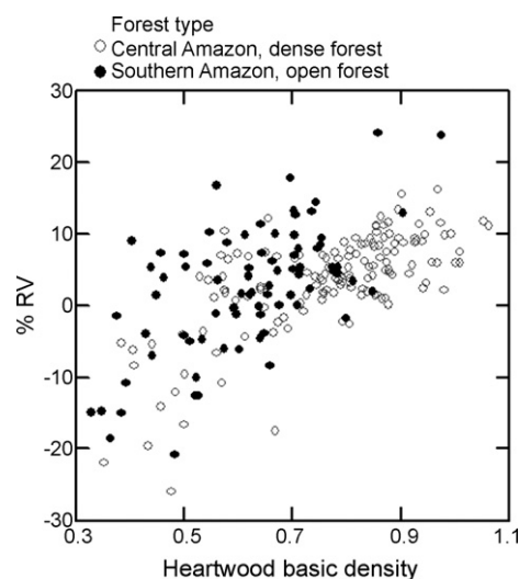
Fig. 2. Percentage difference between basic density of heartwood and of the full disk (%RV) in dense and open forest plotted against heartwood density.
