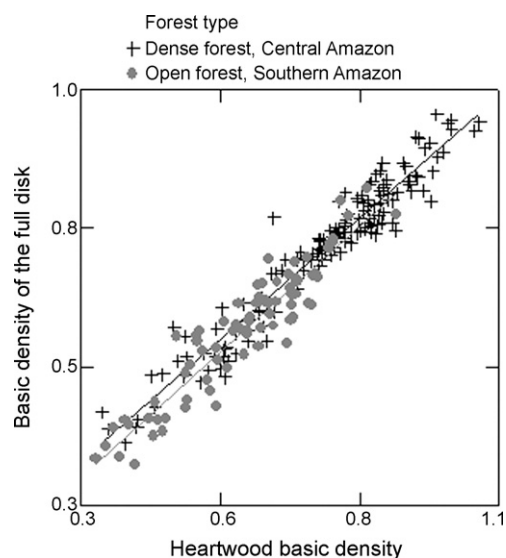
Fig. 1. The relationship between basic density of the full disk and basic density of the heartwood in dense forest in central Amazonia ( n = 146 trees) and in open forest in southern Amazonia ( n = 38 trees).
