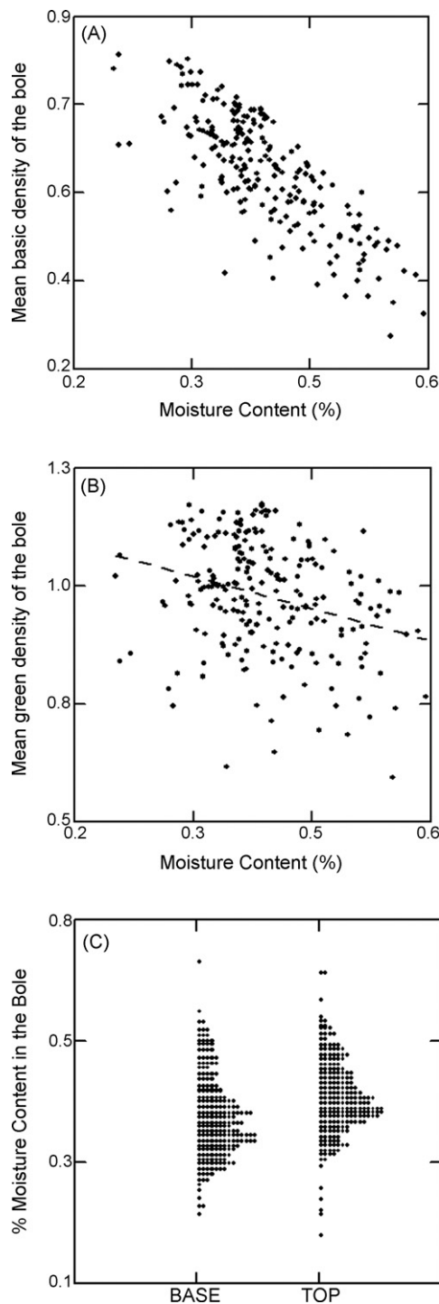
Fig. 5. Relationships between moisture content (%) and mean basic wood density of the bole (A) and between moisture content (%) and mean 'green density' of the bole (B). Variation in moisture content (%) along the length of the bole is also presented (C).
