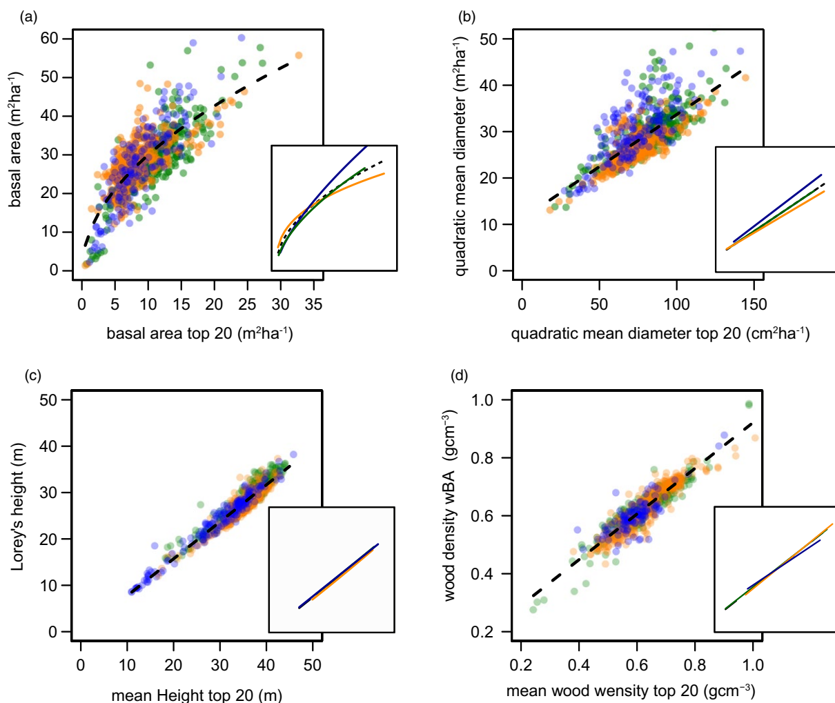
FIGURE 3 Prediction of plot metrics (y axis) from the 20 largest trees (x axis). Results are shown for: (a) basal area, (b) quadratic mean diameter, (c) Lorey's height, and (d) wood density weighted by the basal area. Each dot corresponds to a single plot, coloured in orange, green and blue for America, Africa and Asia, respectively. Both pan-tropical (black dashed lines) and continental (coloured lines) regression models are displayed. These results show that a substantial part of the remaining variance (i.e., not explained by the largest trees) is found when predicting the basal area and the quadratic mean diameter, with slight but significant differences between continents [Colour figure can be viewed at wileyonlinelibrary.com ]
